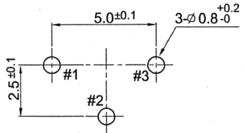
P. C. B MOUNTING HOLE
