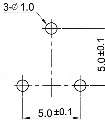
P.C.B MOUNTING
