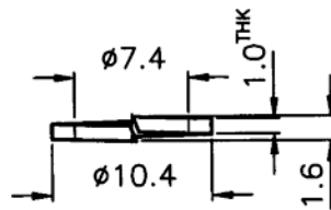
SPRING WASHER
