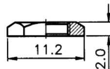
M7X0.75 NUT
