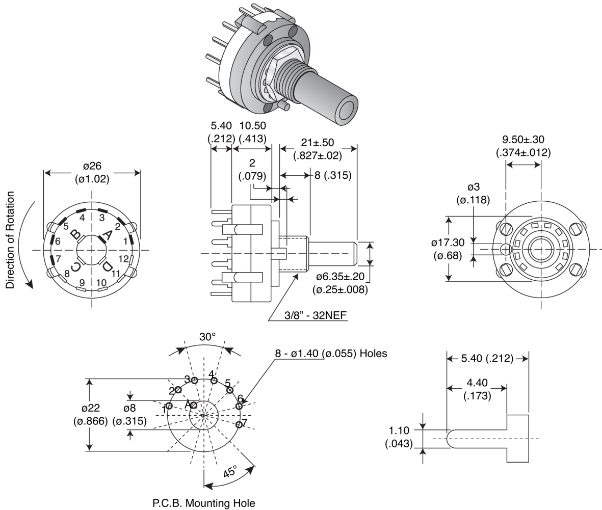
Dimensions mm (In.)
