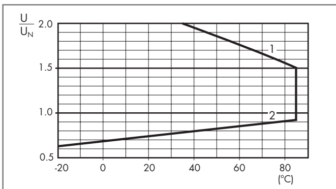
R 44 - DC coil operating range v ambient temperature
